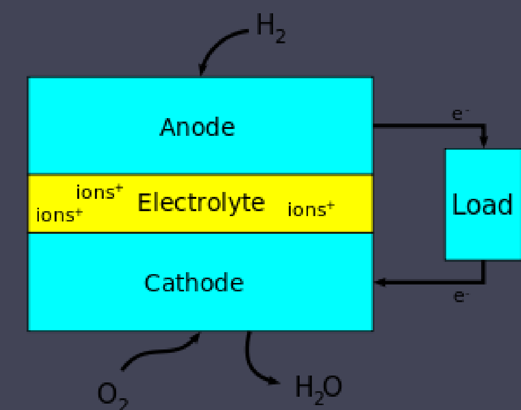
Fig.2 Block diagram of a fuel cell ( \text{H}_2 could also be hydride, methanol, ethanol, formic acid etc.) [ https://en.wikipedia.org/wiki/Fuel_cell ]
