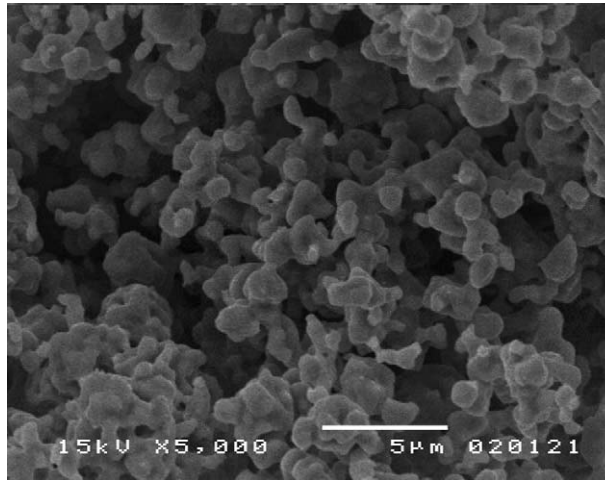
Fig. 5. SEM micrograph of a cobalt powder obtained under static conditions at 800 °C [13].
