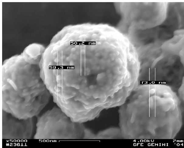
Fig. 8. SEM micrograph of USP cobalt powder obtained at 700 °C with a precursor cobalt concentration of 0.08 mol/l (magnification 50,000×).
