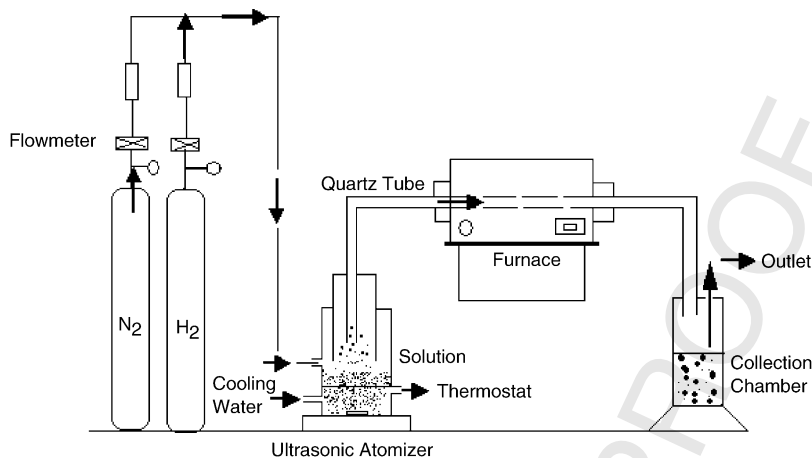
Fig. 1. Schematic drawing of experimental apparatus for the synthesis of cobalt nanoparticles from Co-nitrate-solutions.
