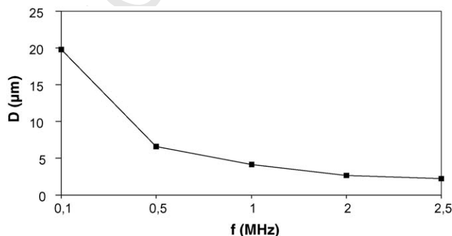
Fig. 6. Dependence of the mean droplet diameter by the frequency of ultrasonic atomizer.
