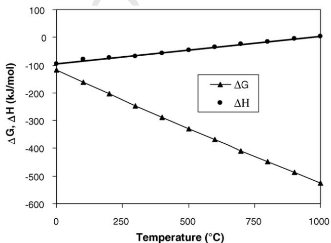
Fig. 3. Dependence of the Gibbs's energy on the temperature.
