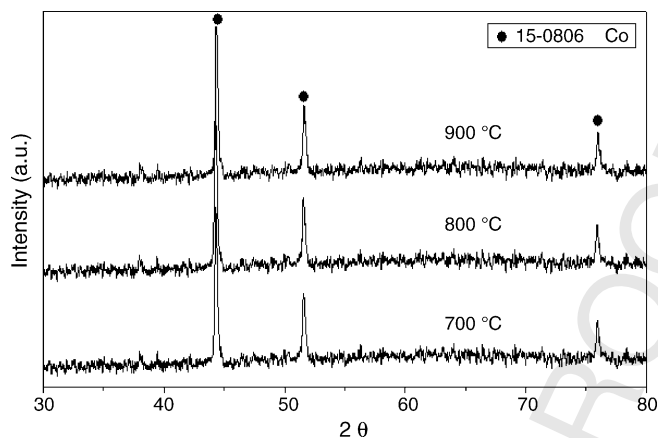
Fig. 2. X-ray analysis of the USP cobalt powders (700, 800 and 900 °C).
