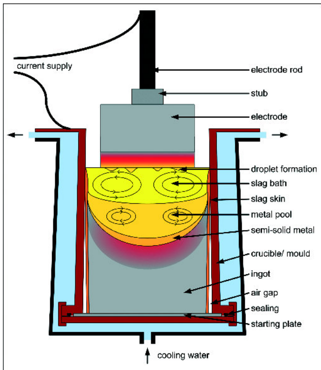
Fig. 1. Principle of the electroslag remelting process.
