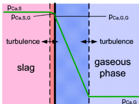
Fig. 9. General model of the transport steps during the evaporation of calcium ( p_{Ca,S} : virtual partial pressure of calcium in the slag; p_{Ca,S,G} : virtual partial pressure of calcium in the slag at the phase boundary; p_{Ca,G,G} : partial pressure of calcium in the gaseous phase at the phase boundary; p_{Ca,G} : partial pressure of calcium in the gaseous phase).
