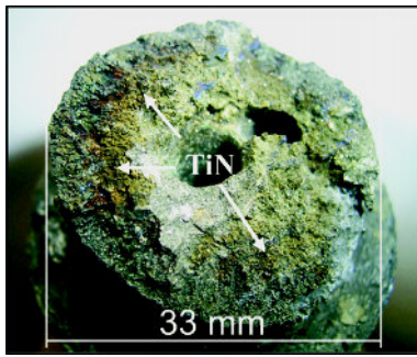
Fig. 7. Formation of TiN in aluminothermic TiAl at the broken electrode surface using a copper mould (electrode head).
