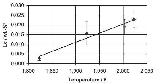
Fig. 3. Solubility product L_c of calcium and oxygen in titanium and TiAl, data. [2]
