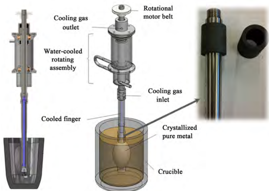
Figure 3. (middle) experimental apparatus of crystallization including “cooled finger” and rotational system, (left) a cross section of the whole unit and (right) steel “cooled finger” with graphite shell.
