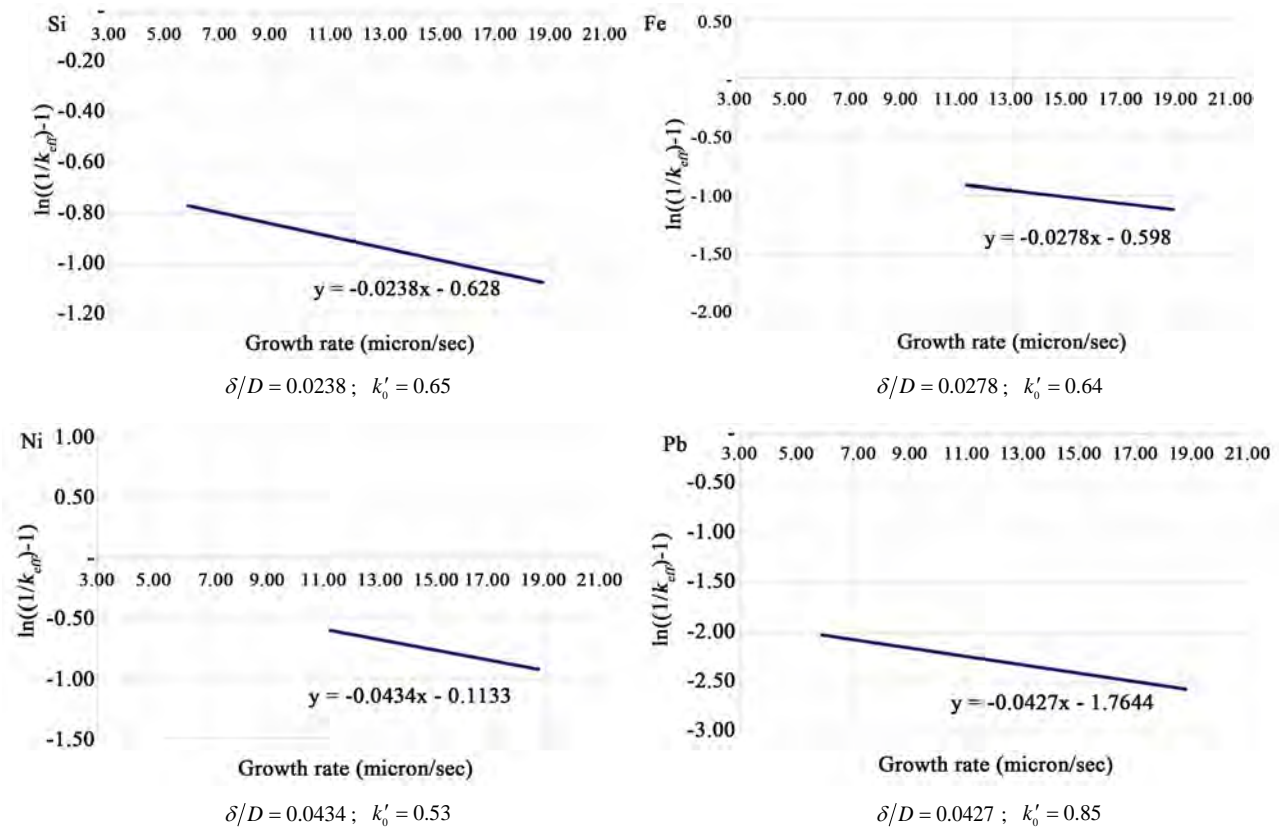
Figure 11. Implementation of the experimental values of C_s and C_L into the BPS model for Silicon, Iron, Nickel and Lead.
