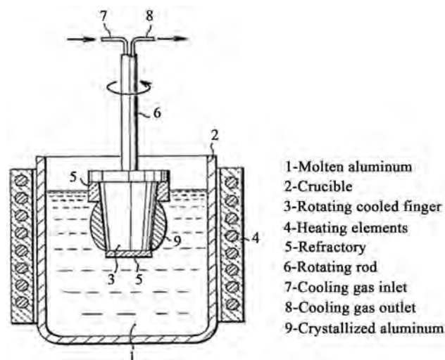
Figure 2. Principle of cooled finger crystallization concept [10].
