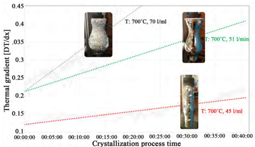
Figure 5. The experimental temperature gradient between the molten bath and the “cooled finger” according to the Process Parameters Melt Temp [ ^{\circ}\text{C} ] as well as cooling gas flow rate (L/min).
