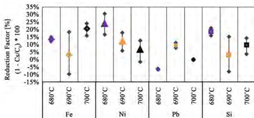
Figure 10. Comparison of the chemical analyses of Aluminum before and after “cooled finger” crystallization of different trials, calculated as reduction factor (%).
