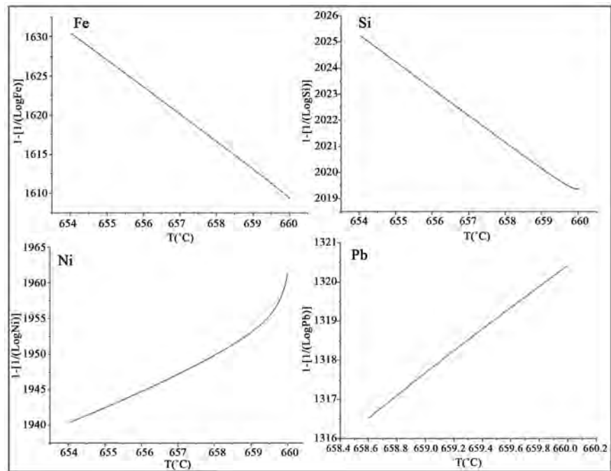
Figure 9. Distribution coefficient of the most common Aluminum impurities versus temperature in the case of a complete mixing, calculated through FactSage.
