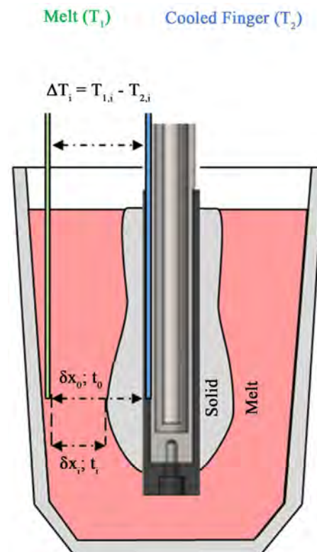
Figure 4. Schematic illustration of Cooled Finger experimental setup, where t_i is the every moment of time, \delta x_i the ever-changing distance between crystallization front and the crucible wall and \Delta T_i the ever-changing temperature difference between the crystallized front and the melt beside the wall.
