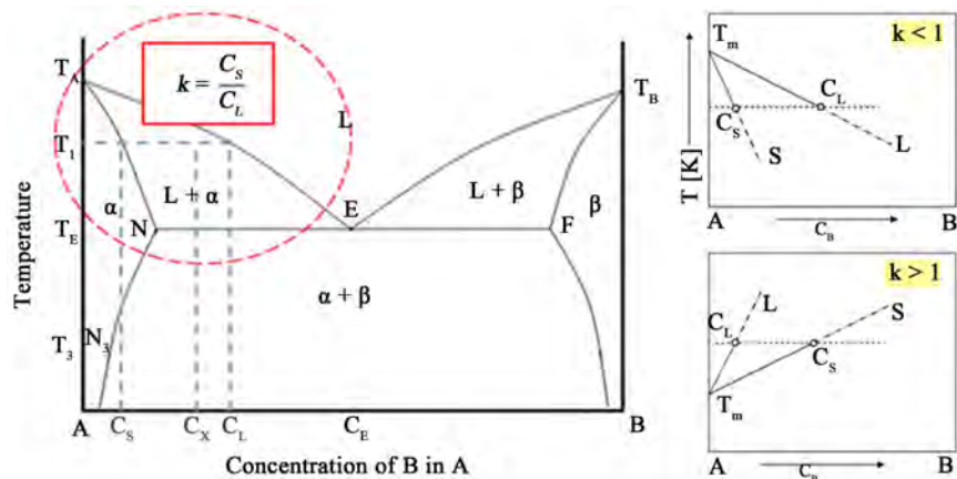
Figure 1. (Left) an exemplary binary phase diagram illustrating the calculation of distribution coefficient and (right) the influence of distribution coefficient on the melting temperature [3].
