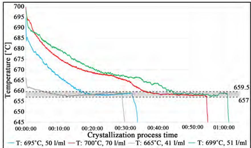
Figure 6. The experimental profile of the crystallization temperature at different initial melt, initial temperature and different cooling gas flow rate without rotation of the “cooled finger”.
