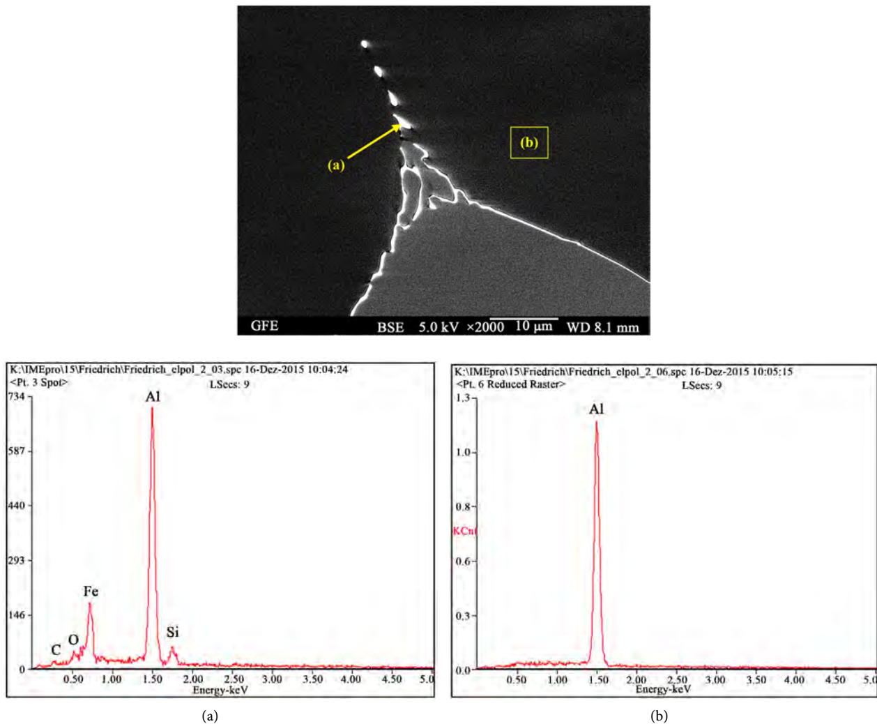
Figure 8. SEM-(top) and EDX-(middle and bottom) pattern of a sample of crystallized Aluminum containing Si and Fe as main impurities, performed via cooled finger methodology.
