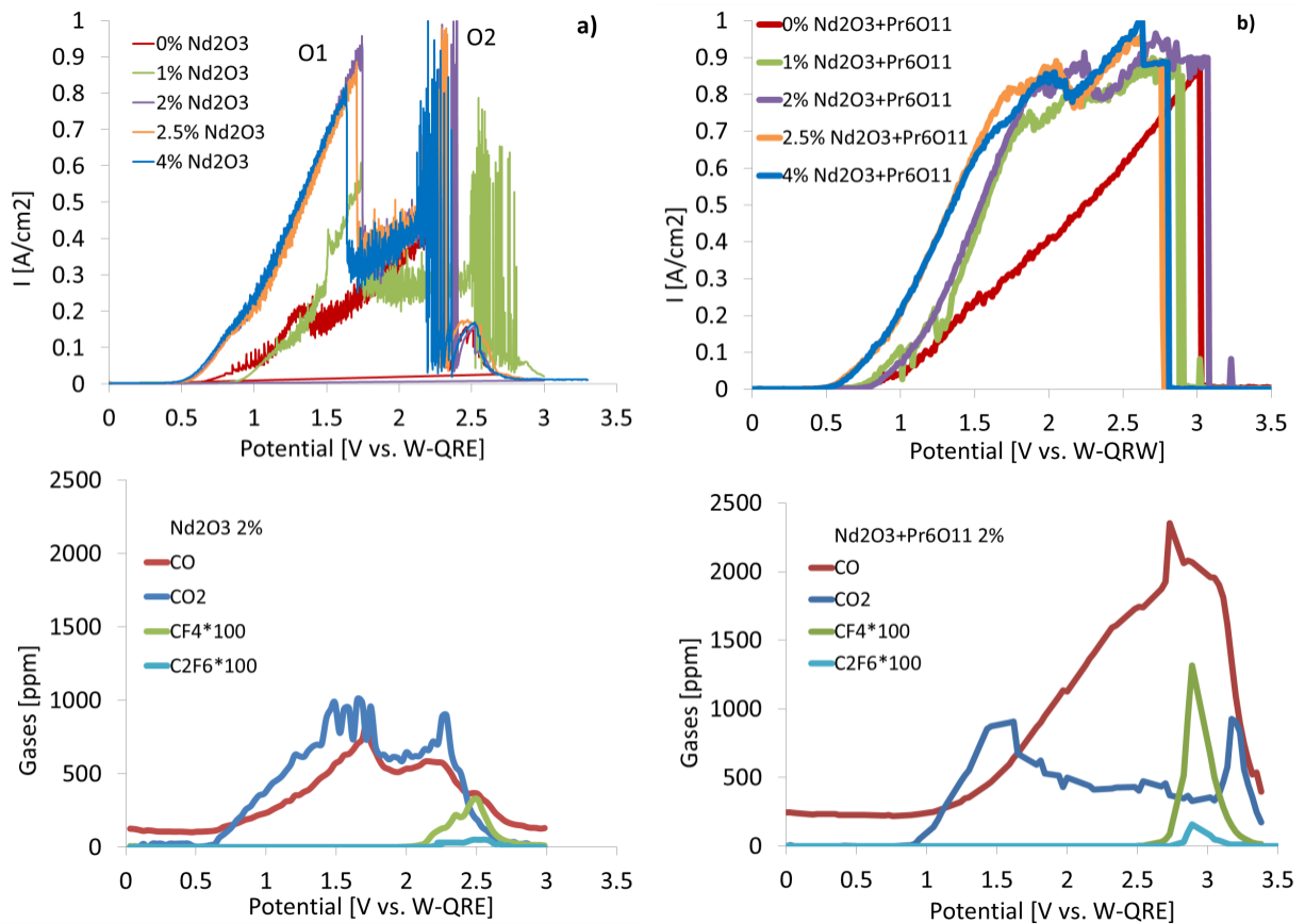
Figure 2: a) Linear sweep voltammograms recorded on graphite electrode at 1050 °C in \text{NdF}_3\text{-LiF} electrolyte with different \text{Nd}_2\text{O}_3 concentrations and scan rate = 5 mV/s (above) with off-gases measured with an in-situ FTIR-spectrometer generated during electrochemical measurements with 2 wt.-% oxide (below); b) Linear sweep voltammograms recorded on graphite electrode at 1050 °C in \text{NdF}_3\text{-PrF}_3\text{-LiF} electrolyte with different \text{Nd}_2\text{O}_3 - \text{Pr}_6\text{O}_{11} concentrations and scan rate v = 5 mV/s (above) with off-gases measured with in-situ FTIR-spectrometer generated during electrochemical measurements with 2 wt.-% oxide (below).
