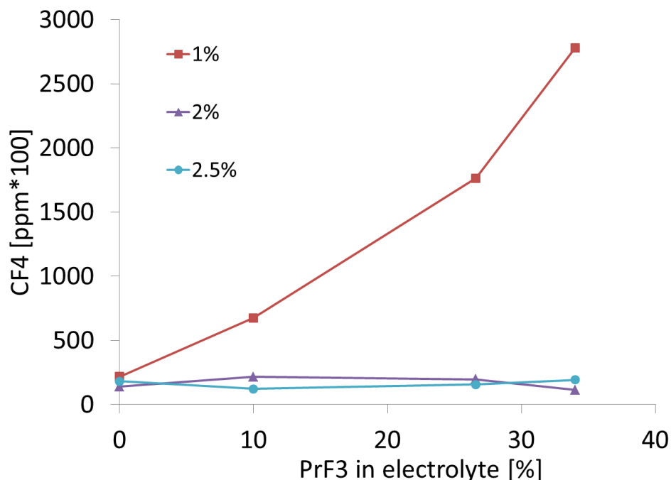
Figure 3: Maximum \text{CF}_4 concentration in ppm*100 in off-gas during electrochemical measurements in different \text{NdF}_3\text{-PrF}_3\text{-LiF} electrolyte systems with increasing praseodymium percentage and with different oxide amounts at 1050 °C measured by FTIR-spectrometer
