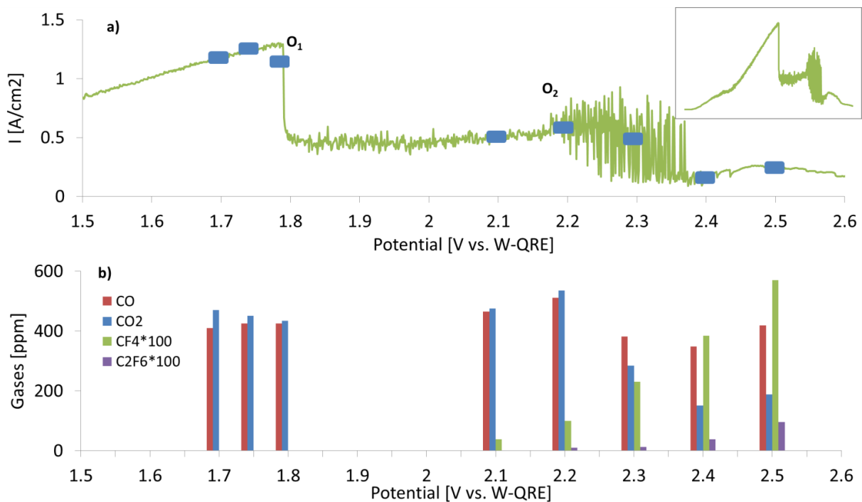
Figure 5: a) Chosen potentials for chronoamperometry presented on linear sweep voltammogram of \text{NdF}_3\text{-PrF}_3\text{-LiF} (64.23 - 23.27 -12.5 wt.-%) system with 1 wt.-% \text{Nd}_2\text{O}_3 - \text{Pr}_2\text{O}_3 (whole voltammogram in inset). b) Off-gas composition during the chronoamperometry on potentials marked in figure a).
