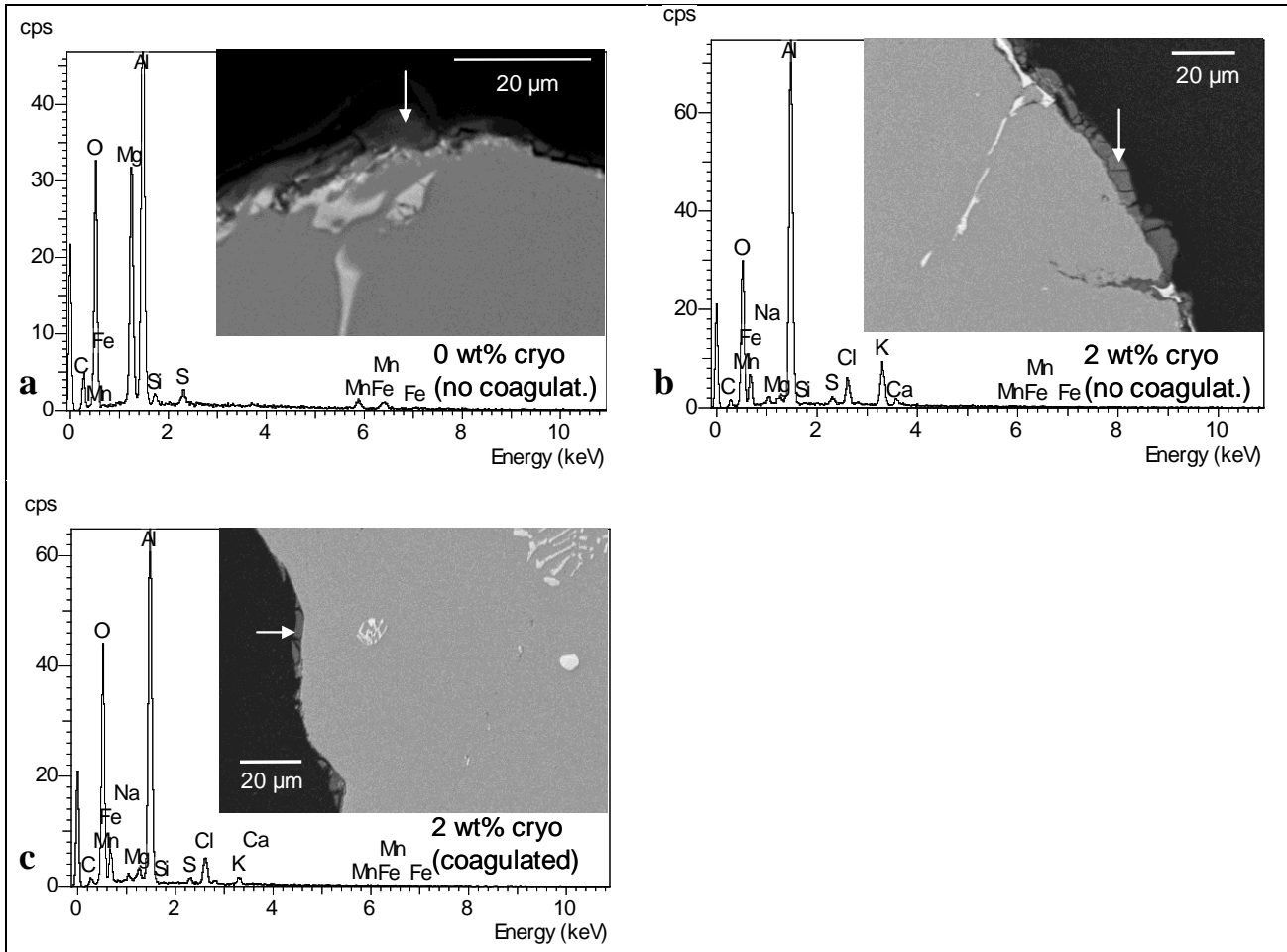
Figure 8: SEM (BSE) observation of the section of the solidified droplets for AA3104, T_{initial}=800^{\circ}\text{C} (a- bead <2.5 mm 0 wt% cryolite; b- bead < 2.5 mm 2 wt% cryolite, c- bead >2.5 mm 2 wt% cryolite)
