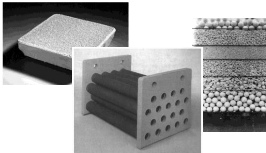
Figure 4. Filter devices for Aluminium melt filtration (from left to right: CFF, RMF, BF)
