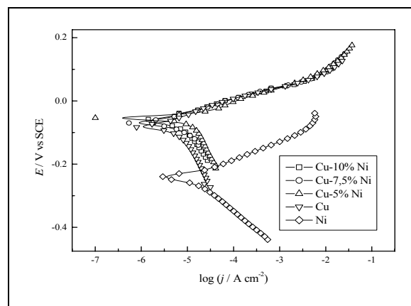
Fig.1. Corrosion behavior of different anode samples in sulphuric acid solution
